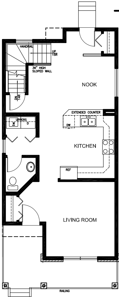
MAIN FLOOR 737 SQ. FT.
