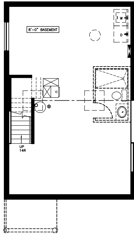
FOUNDATION PLAN
