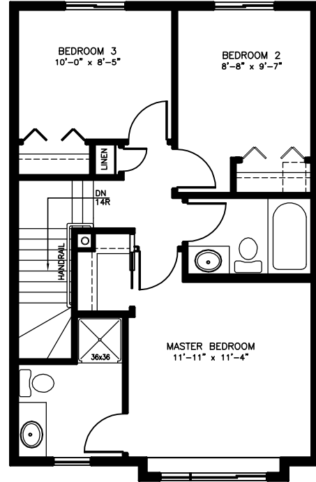
SECOND FLOOR 600 SQ. FT.
