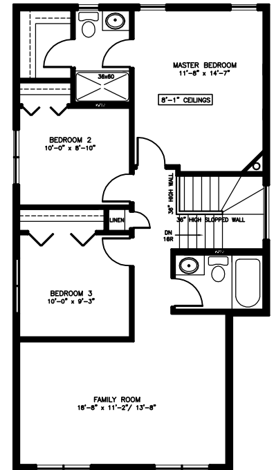
THREE BEDROOM PLUS FAMILY ROOM
